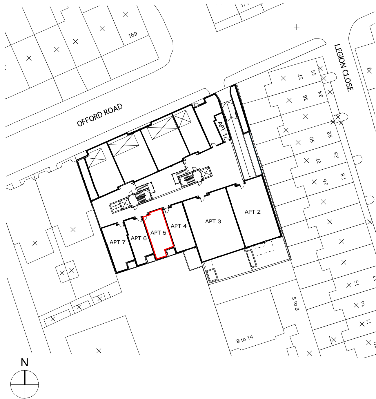
GROUND FLOOR PLAN SCALE 1:500 @ A3
